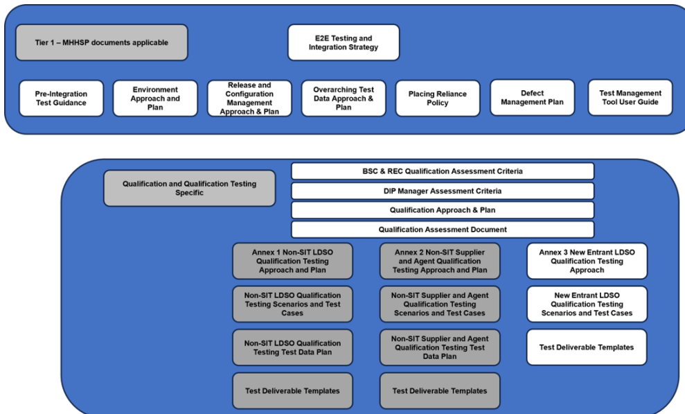
Figure 1: Document Hierarchy
